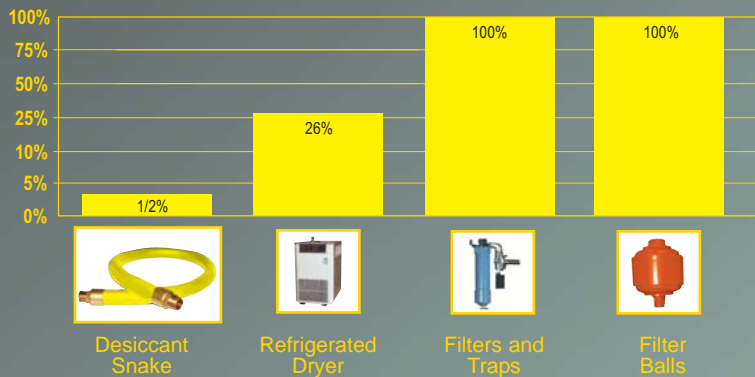
Relative Humidity remaining in the compressed air after treatment†
